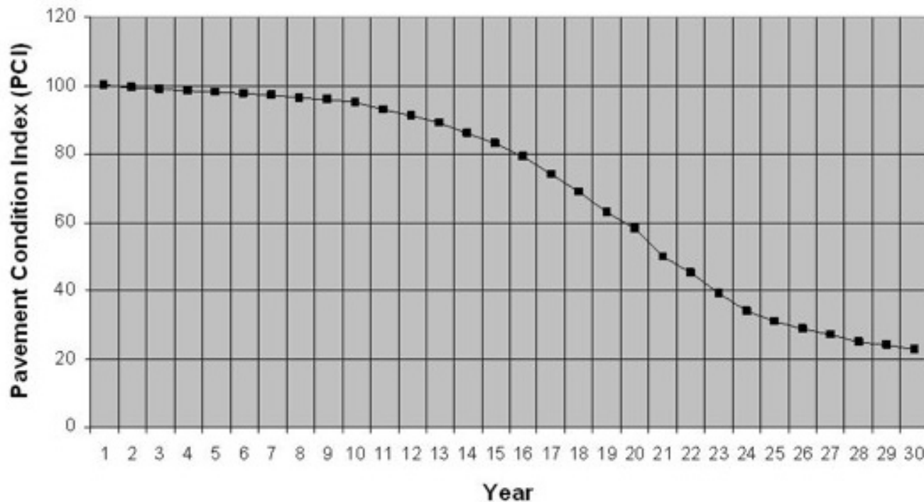
Typical Parking Lot Pavement Lifecycle
